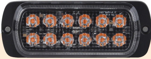
L 114 x W 43.4 x H 12.5mm 12-LED AMBER | Part no. 0-441-74
