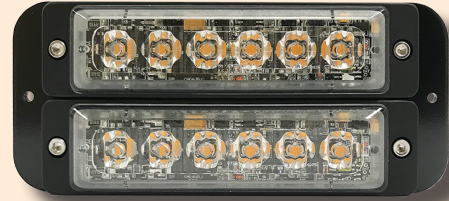
L 133 x W 56.8 x H 12.6mm 12-LED AMBER | Part no. 0-441-10
